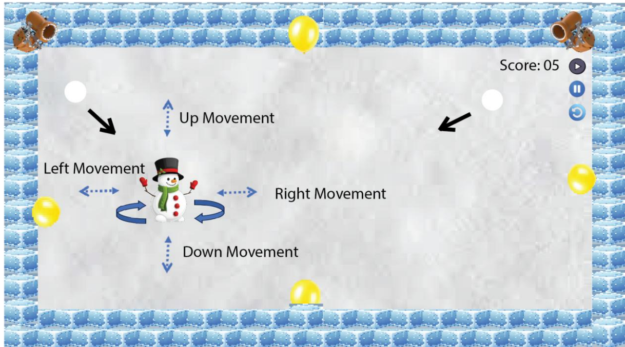
Figure 2: Game Arena
